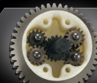
Planetary Differential
